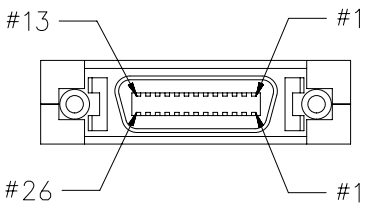
CN1 CAMERA SIDE
