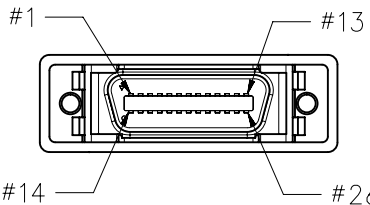
CN2 FRAME GRABBER BOARD SIDE
